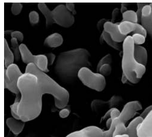
TCPOP-05 \beta -TCP Powder for Orthopedic APS 0.5 \mu m & 3 \mu m Purity ≥ 99.0%.
